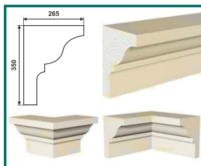
КН-350/3 (350 × 265 × 2000)
