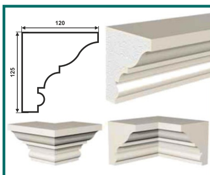
KH-125/1 (125 × 120 × 2000)
