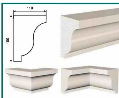
KH-160/1 (160 × 110 × 2000)
