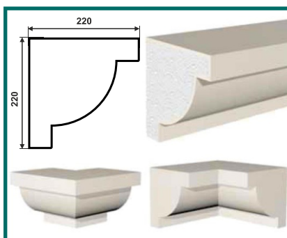
KH-220/5 (220 × 220 × 2000)
