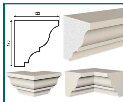
KH-126/1 (126 × 122 × 2000)
