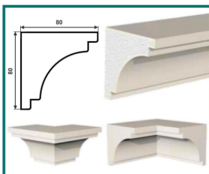
KH-80/1 (80 × 80 × 2000)
