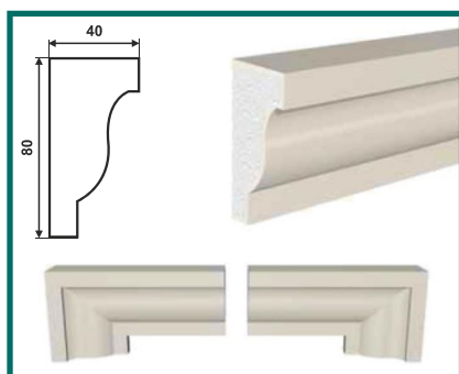
МД-80/2 (80 × 40 × 2000)
