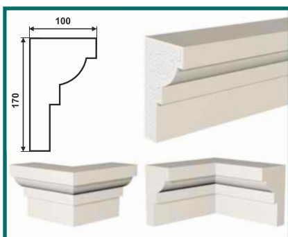
KH-170/2 (170 × 100 × 2000)
