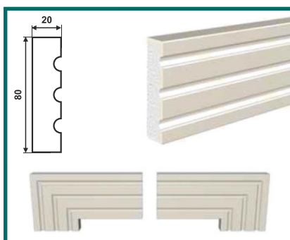
МД-80/3 (80 × 20 × 2000)
