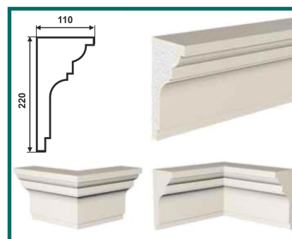
KH-220/3 (220 × 110 × 2000)
