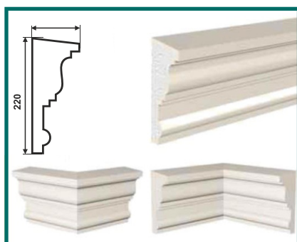
KH-220/1 (220 × 90 × 2000)
