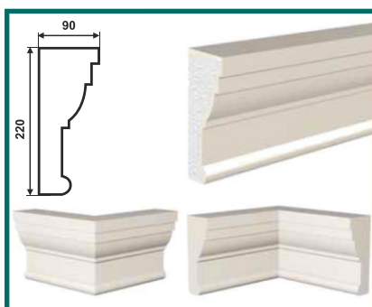
KH-220/2 (220 × 90 × 2000)
