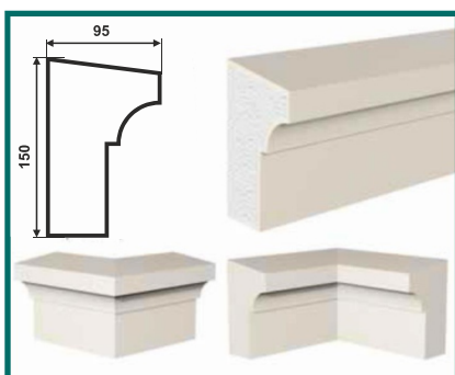
KH-150/4 (150 × 95 × 2000)
