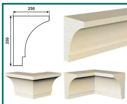
КН-350/2 (350 × 250 × 2000)
