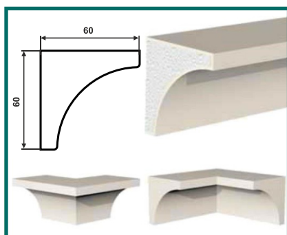
KH-60/1 (60 × 60 × 2000)
