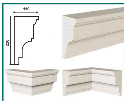
KH-220/4 (220 × 110 × 2000)
