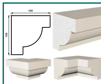
KH-100/1 (100 × 100 × 2000)
