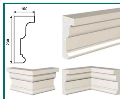
KH-230/1 (230 × 100 × 2000)
