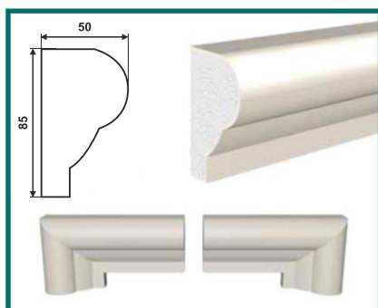
МД-85/1 (85 × 50 × 2000)
