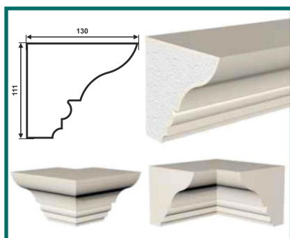
KH-111/1 (111 × 130 × 2000)
