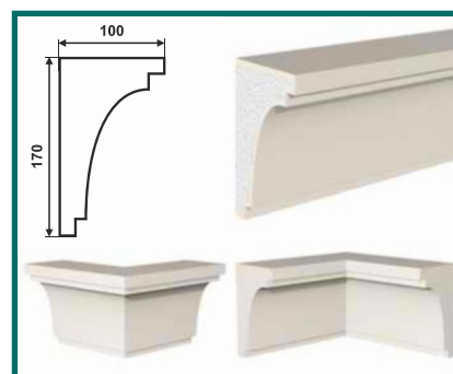
KH-170/1 (170 × 100 × 2000)
