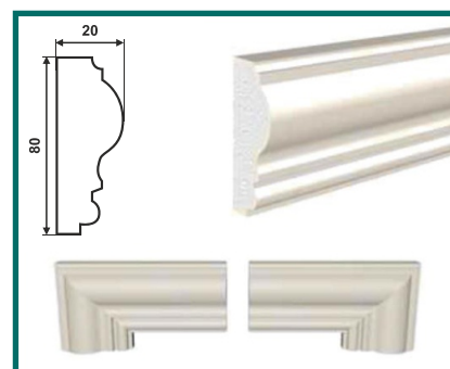
МД-80/4 (80 × 30 × 2000)
