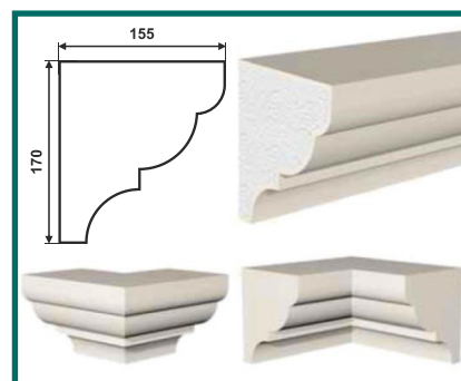
KH-170/4 (170 × 155 × 2000)
