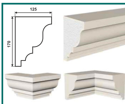
KH-170/3 (170 × 125 × 2000)
